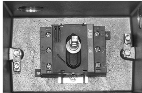
Internal view showing DIN rail mounted ABB OT63F3 non-Fusible, heavy duty, disconnect switch with dual grounding lugs and actuation shaft.
